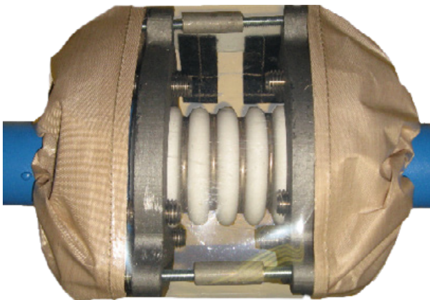
Glassfibre Coated PTFE shield with FEP Window
